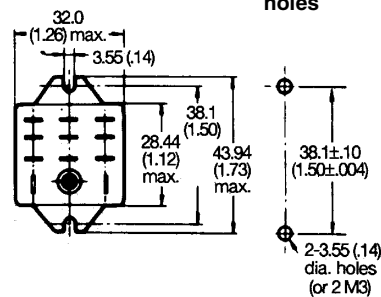
Mounting holes
