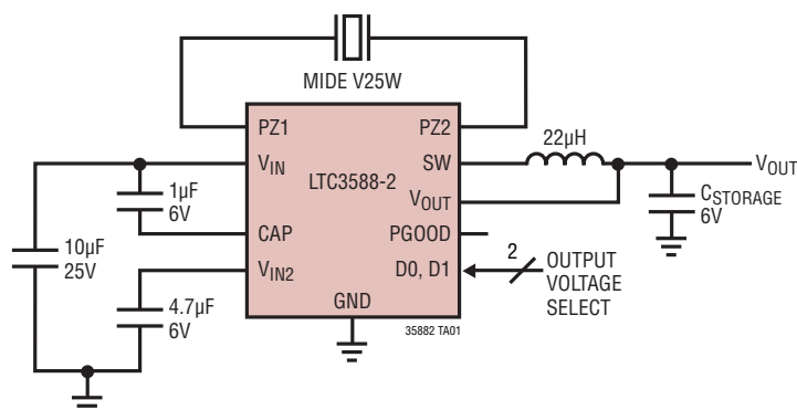
High Voltage Piezoelectric Energy Harvesting Power Supply
