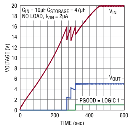
LTC3588-2 5.0V Regulator Start-Up Profile
