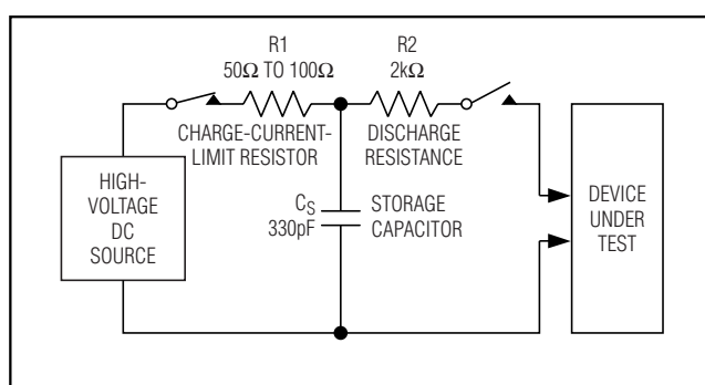
Figure 13. ISO 10605 Contact Discharge ESD Test Circuit
