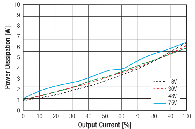
Power Dissipation vs. Output Current
