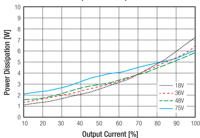
Power Dissipation vs. Output Current
