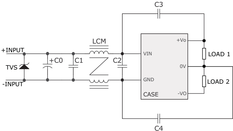
Figure 2 (Dual output)
