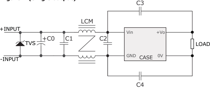
Figure 1 (Single output)
