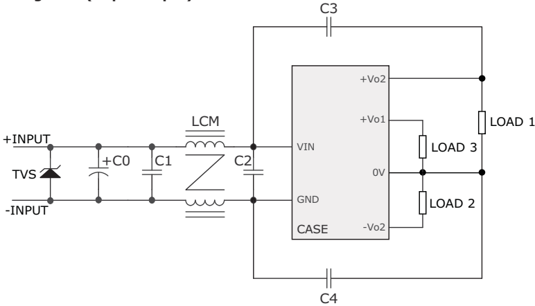
Figure 3 (Triple output)
