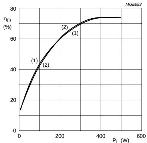
Class-B operation; V_{DS} = 50\text{ V} ; I_{DQ} = 2 \times 0.1\text{ A} ; f = 108\text{ MHz} ; Z_L = 3.2 + j4.3\ \Omega (per section); R_{GS} = 4\ \Omega (per section). (1) T_h = 25\text{ }^\circ\text{C} . (2) T_h = 70\text{ }^\circ\text{C} .
