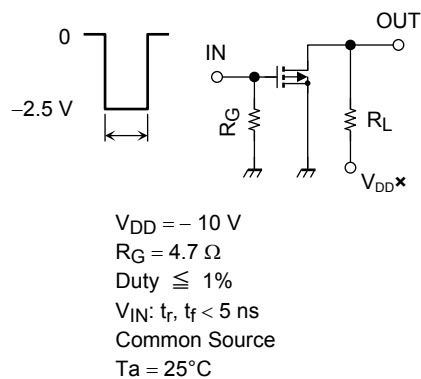
(a) Test circuit
