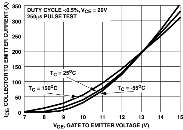
FIGURE 13. TRANSFER CHARACTERISTIC
