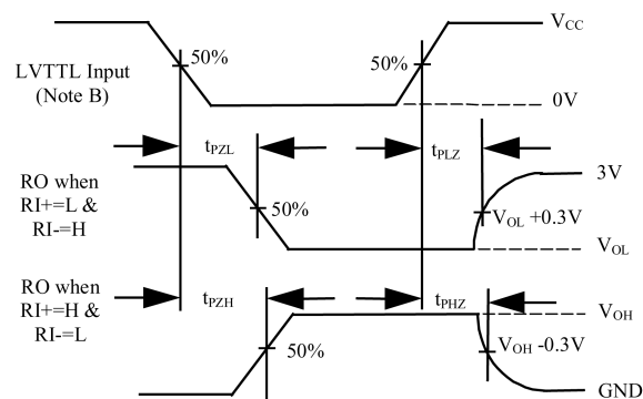
FIGURE 3. LVTTTL Outputs Test Circuit and AC Waveforms
