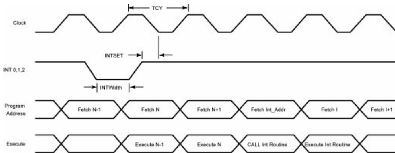
Figure 11. Interrupt Timing
