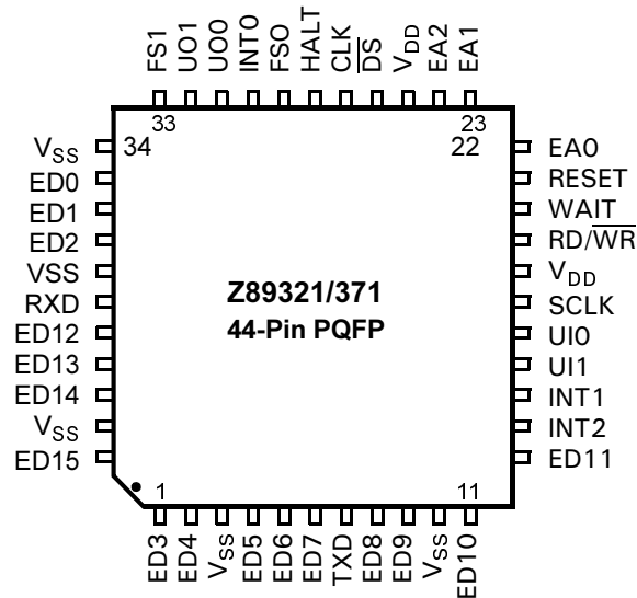
Figure 5. Z89321/371 44-Pin PQFP Pin Assignments
