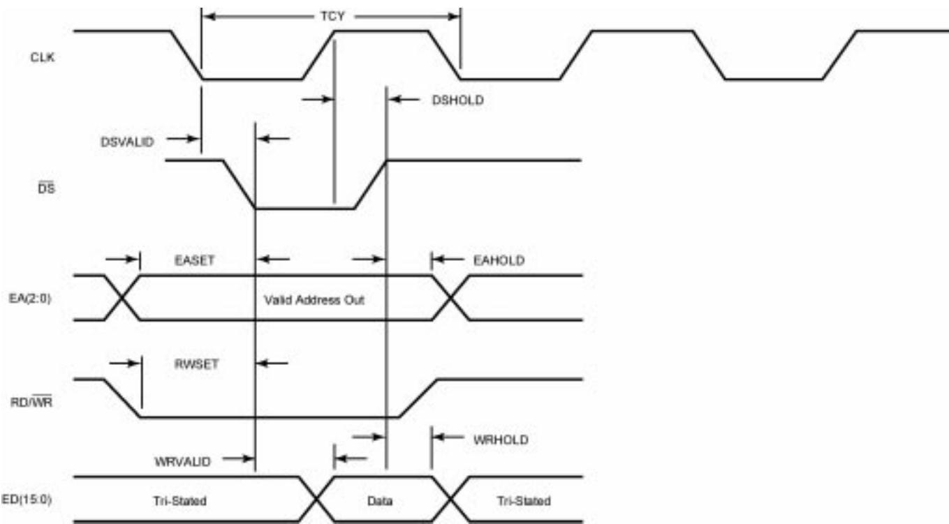
Figure 9. Write Timing
