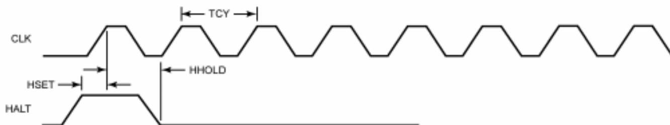
Figure 12. HALT Timing
