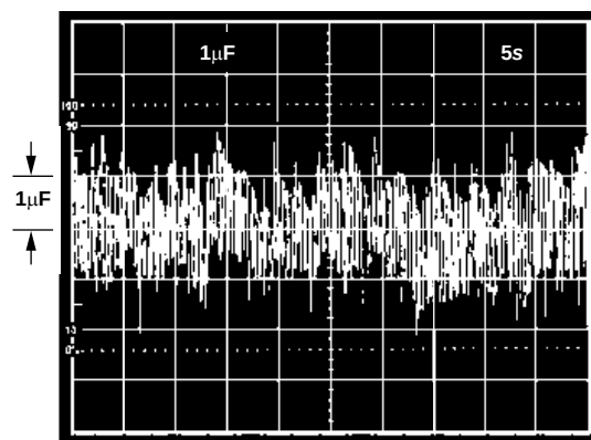
Figure 7. 0.1 Hz to 10 Hz Noise
