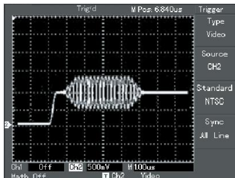
Figure 2-14 Video trigger: line synchronization
