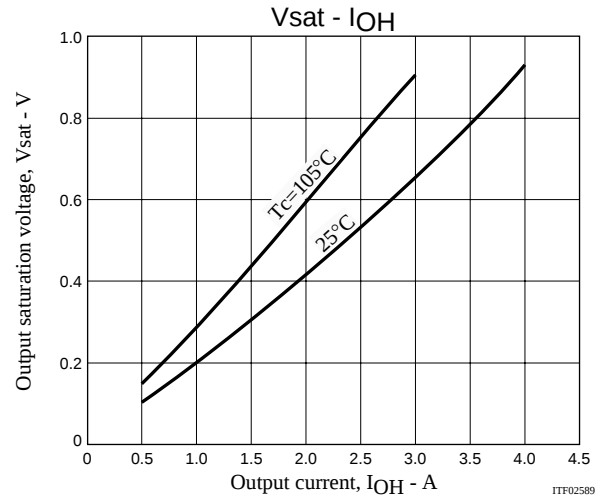
STK672-640A-E Output saturation voltage, V_{sat} - Output current, I_{OH}
