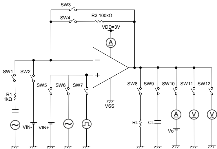
Figure 72. Test circuit 2
