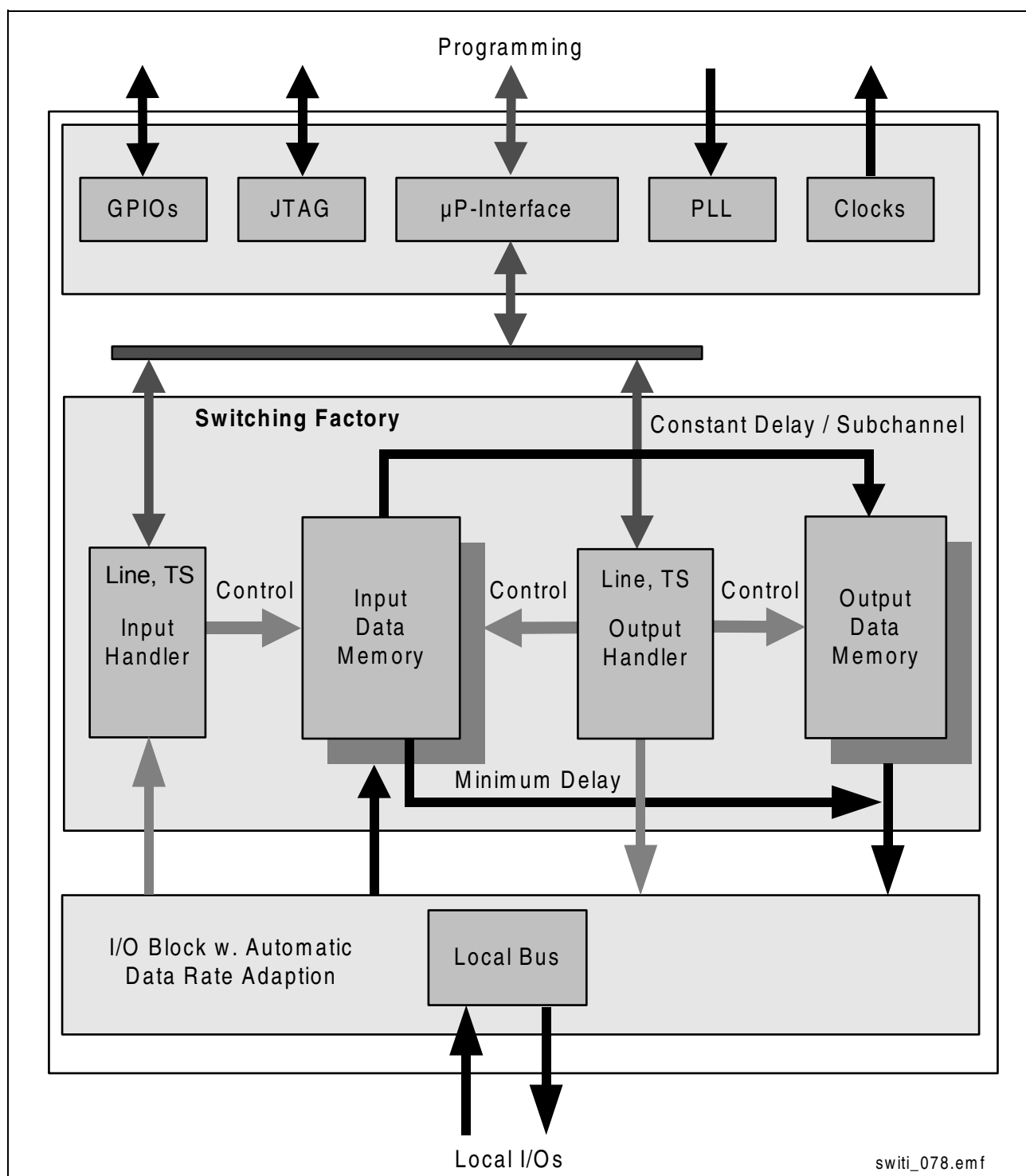
Figure 4 Block Diagram
