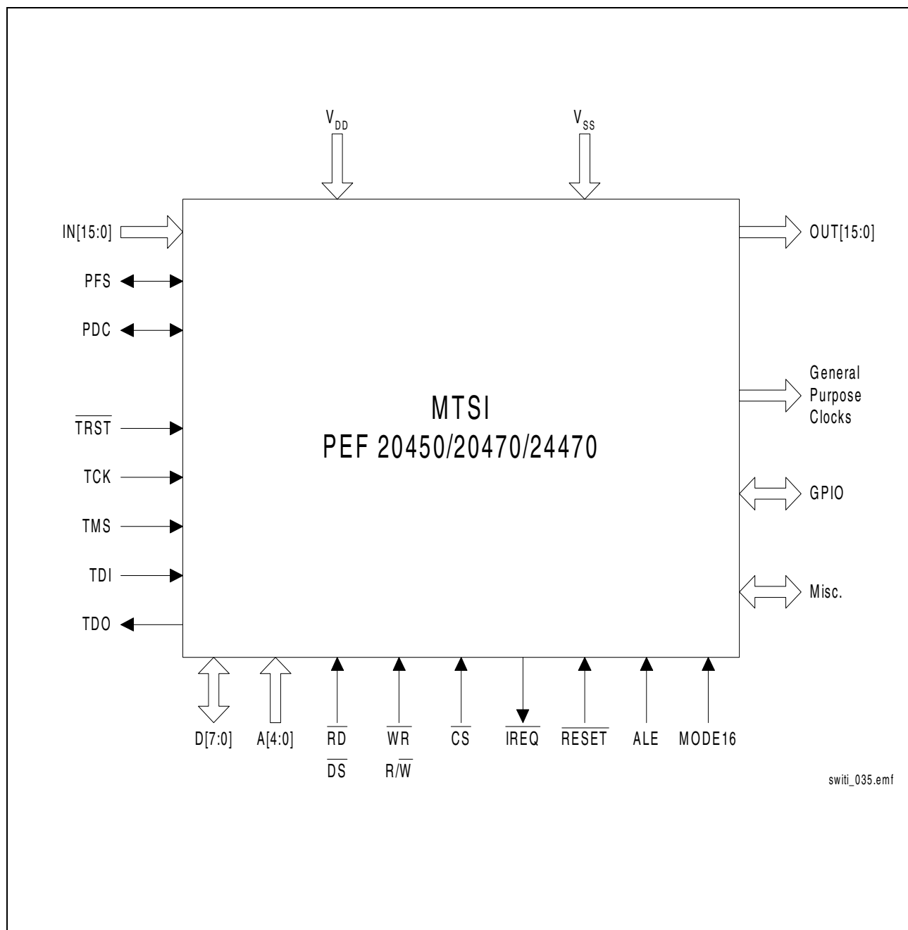
Figure 1 Logic Symbol
