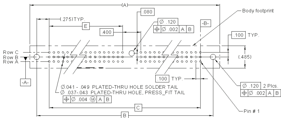
Recommended PCB hole mounting pattern
