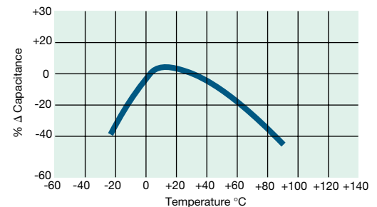
Temperature Coefficient
