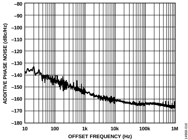
Figure 17. Additive Phase Noise vs. Offset Frequency RF Frequency = 12 GHz at Small Signal
