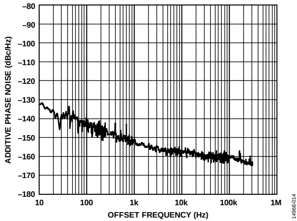
Figure 16. Additive Phase Noise vs. Offset Frequency RF Frequency = 12 GHz, RF Input Power = 3 dBm ( P_{1dB} )
