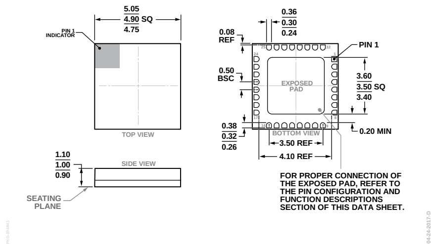
Figure 21. 32-Terminal Ceramic Leadless Chip Carrier [LCC] (E-32-1)
