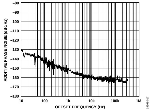
Figure 18. Additive Phase Noise vs. Offset Frequency, RF Frequency = 12 GHz, RF Input Power = 11 dBm ( P_{SAT} )
