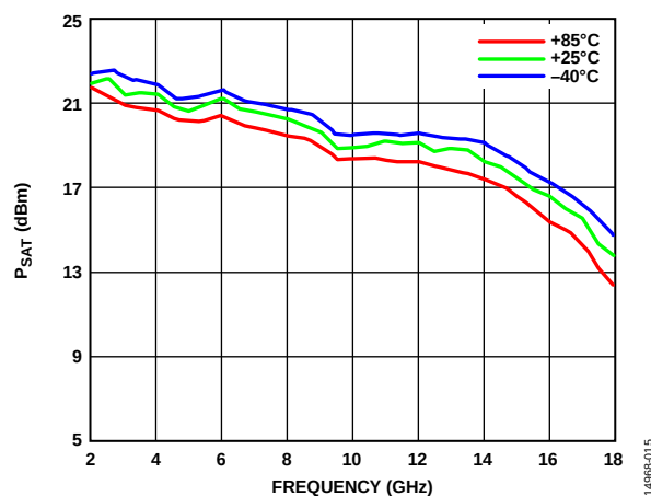
Figure 15. Saturated Power ( P_{SAT} ) vs. Frequency for Various Temperatures
