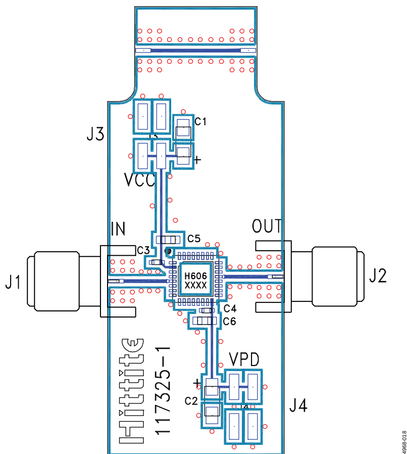
Figure 20. Evaluation PCB
