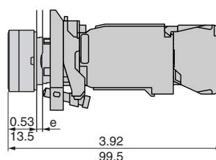
Illuminated selector switches Protected LED XB4BK12••5
