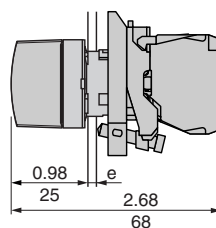
Illuminated selector switches Protected LED XB4BK12••5
