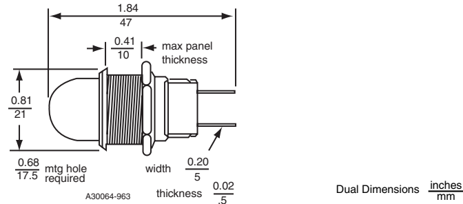
Approximate Dimensions
