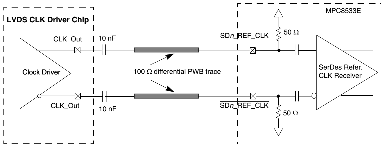
Figure 46. AC-Coupled Differential Connection with LVDS Clock Driver (Reference Only)
