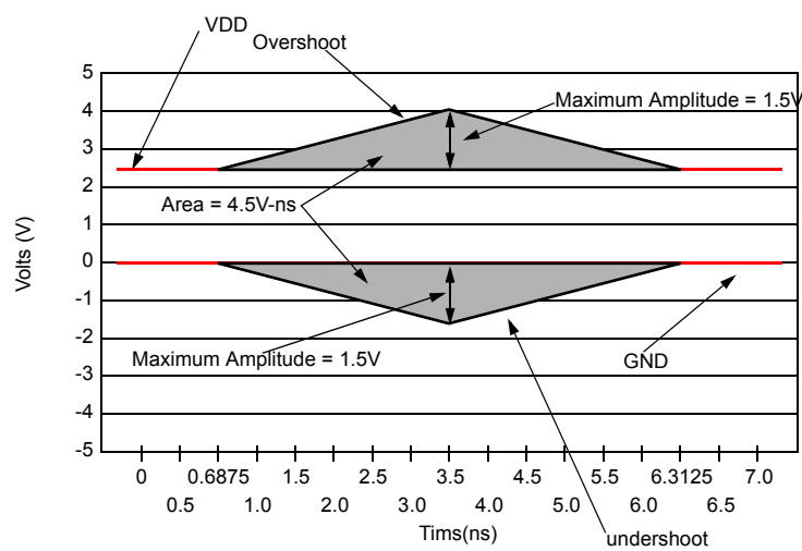
AC overshoot/Undershoot Definition
