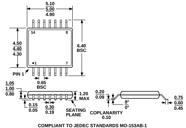
Figure 61. 14-Lead Thin Shrink Small Outline Package [TSSOP] (RU-14)
