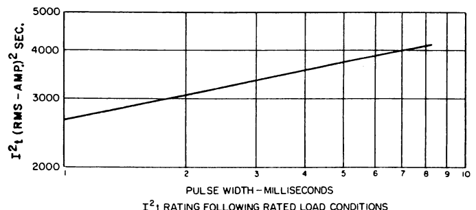
6. MAXIMUM ALLOWABLE NON-REPETITIVE SURGE CURRENT
