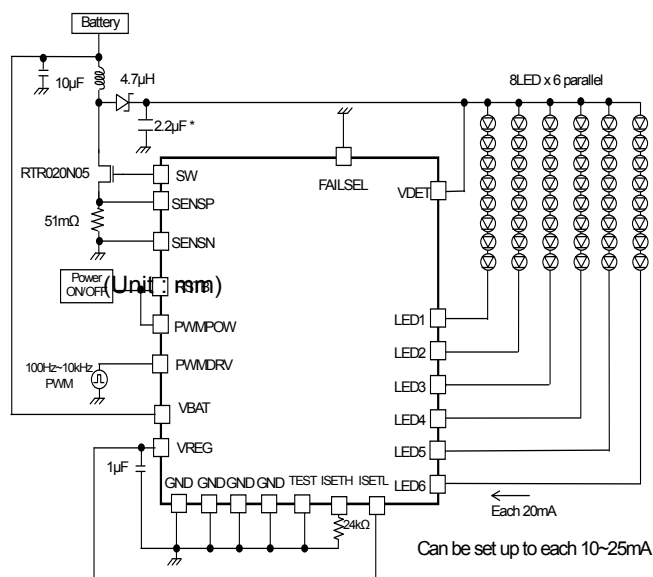
Fig.46 8 series × 6 parallel, LED current 20mA setting Current driver PWM application
