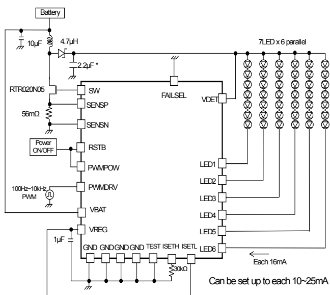
Fig.47 7 series × 6 parallel, LED current 16mA setting Current driver PWM application
