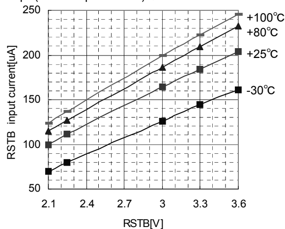
Fig .34 RSTB terminal voltage-RSTB inflow current (At the time of the current driver six lines use)
