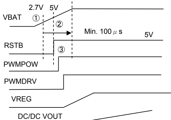
Figure.31 control Signal timing
