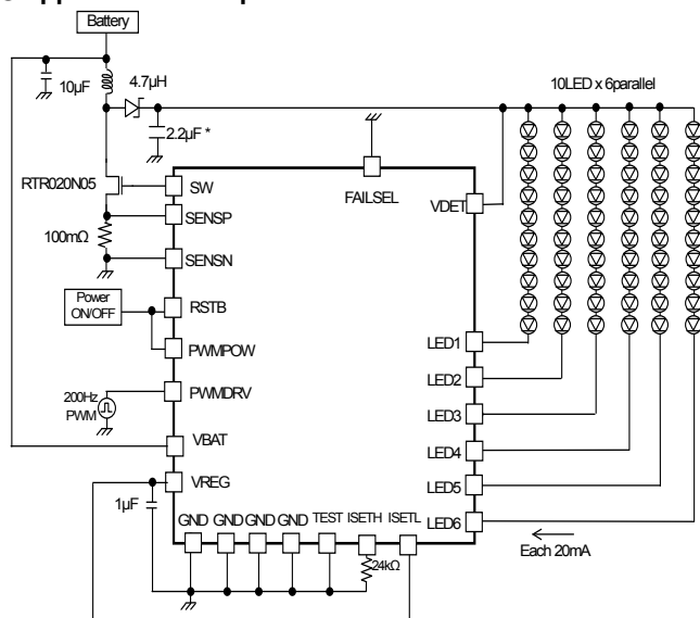
Fig.25 10 series x 6parallel Hi current 20mA setting Current driver PWM application
