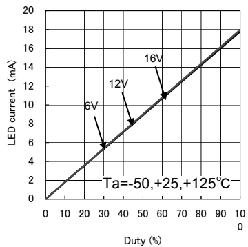
Fig.7 LED current vs PWMDRV-HI Duty PWM = 200Hz
