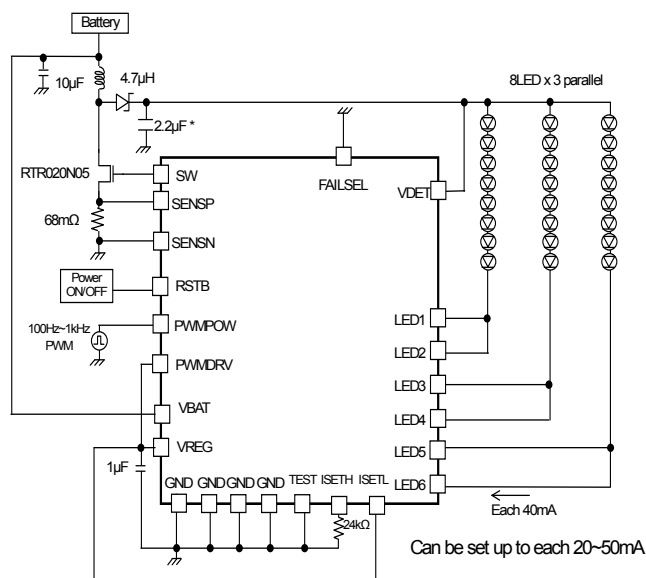
Fig.52 8 series × 3 parallel, LED current 40mA setting Power control PWM application
