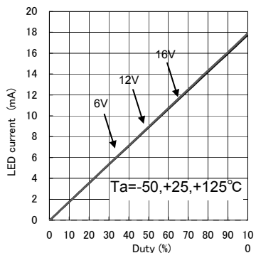
Fig.10 LED current vs PWMPOW-HI Duty TPWM = 200Hz
