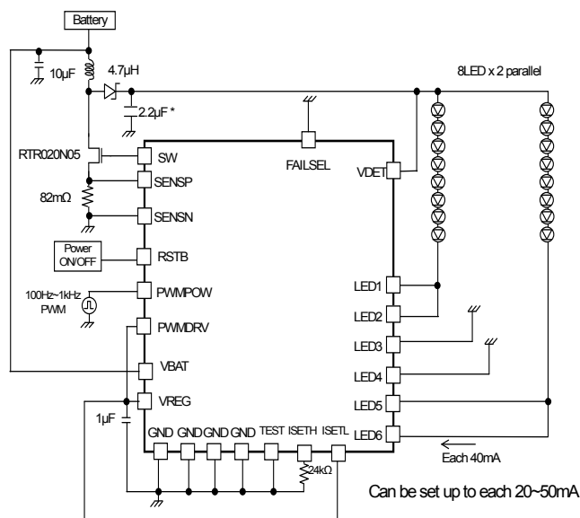
Fig.54 8 series × 2 parallel, LED current 40mA setting Power control PWM application
