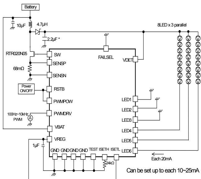
Fig.49 8 series × 3 parallel, LED current 20mA setting Current driver PWM application
