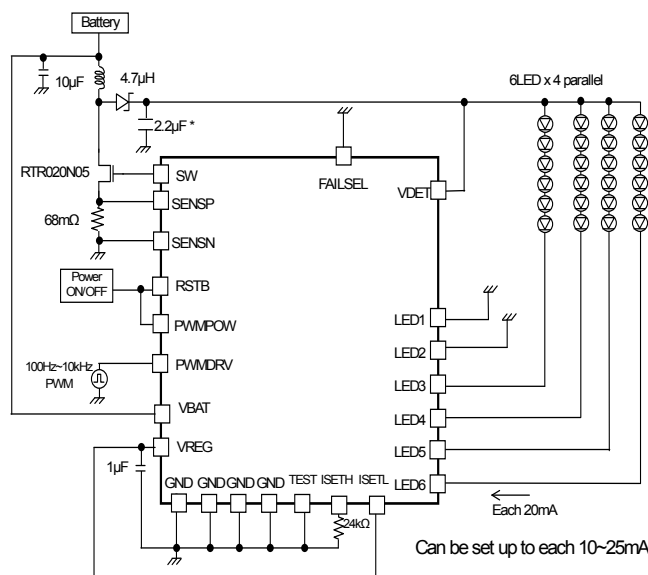
Fig.50 6 series × 4 parallel, LED current 20mA setting Current driver PWM application
