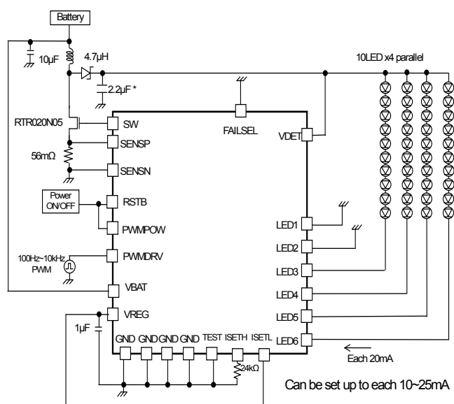
Fig.48 10 series × 4 parallel, LED current 20mA setting Current driver PWM application
