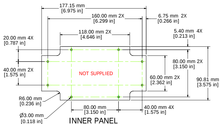
INNER PANEL
