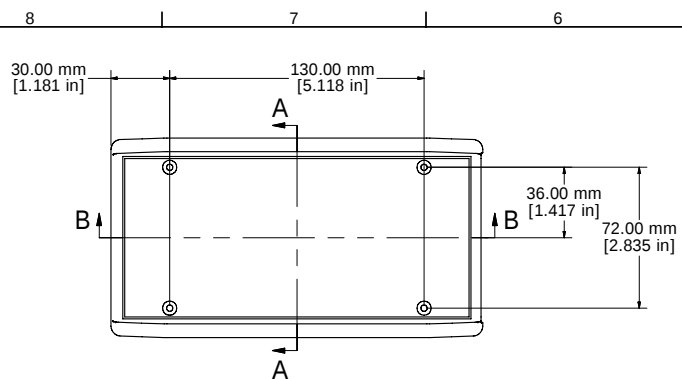
ASSEMBLY - TOP
