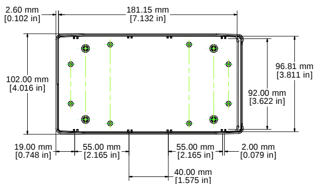
BOX - INSIDE
