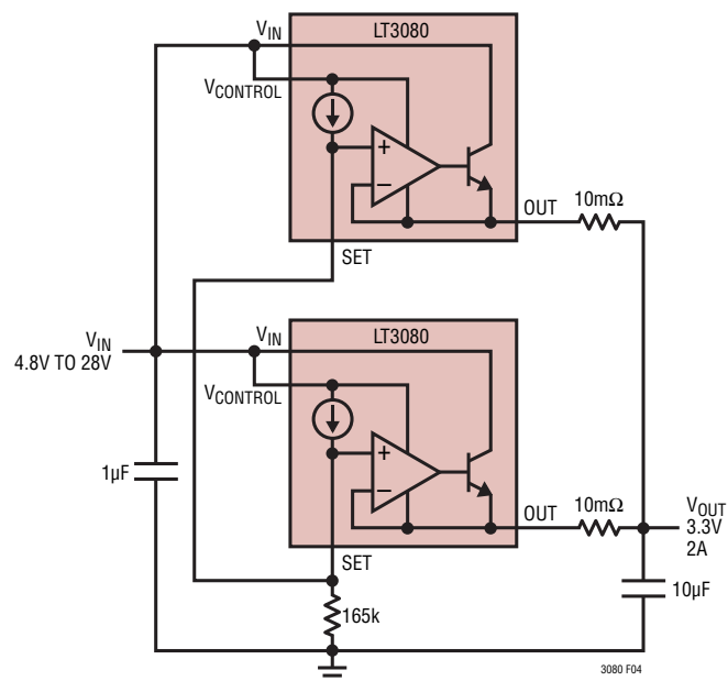
Figure 4. Parallel Devices
