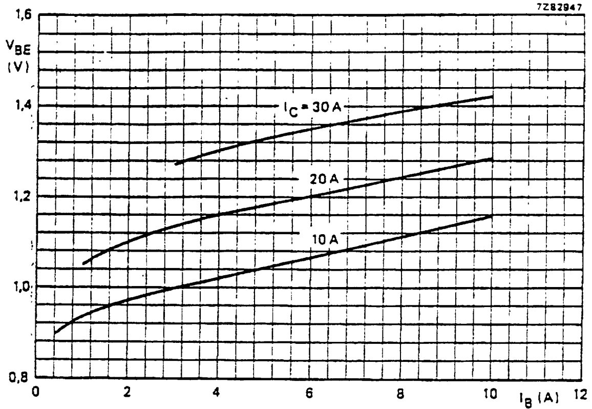
Fig. 14 Typical values at T_j = 25 °C.
