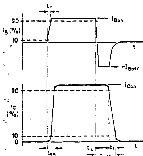
Fig. 5 Switching times waveforms with resistive load.
