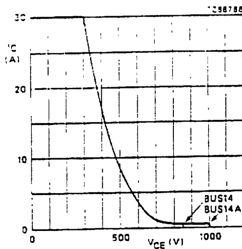
Fig. 10 Reverse bias SOAR.
