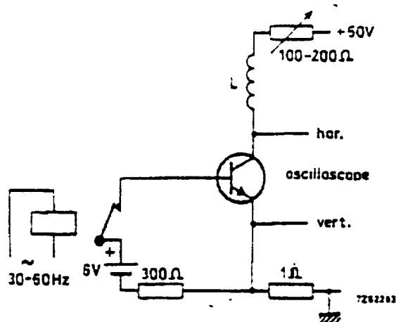
Fig. 3 Test circuit for V_{CEOsust} .
