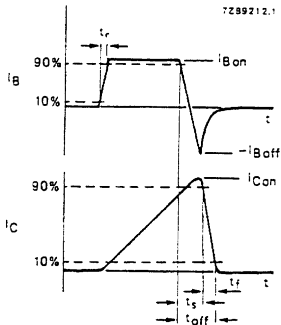
Fig. 6 Switching times waveforms with inductive load.
