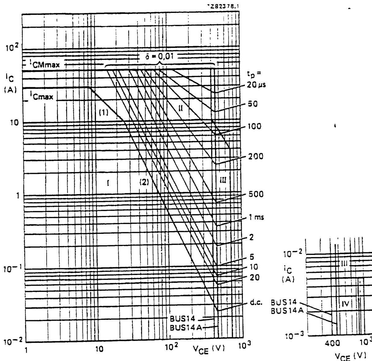
Fig. 8 Safe Operating Area at T_{mb} \leq 25^{\circ}\text{C} .
