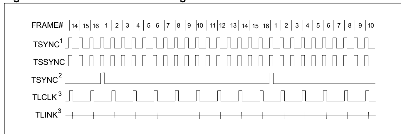
Figure 31-18. Transmit-Side Timing
