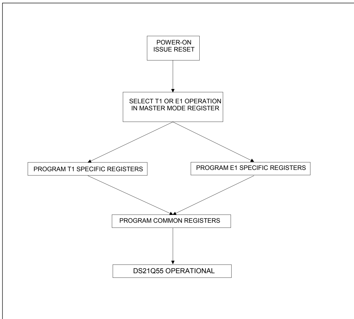
Figure 5-1. Programming Sequence
