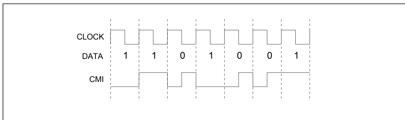
Figure 22-2. CMI Coding
