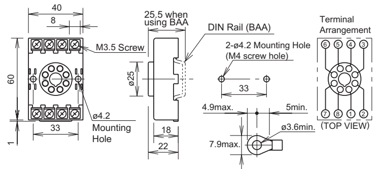
8-Pin SR2P-06
