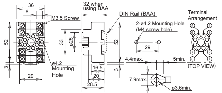
8-Pin SR2P-05
