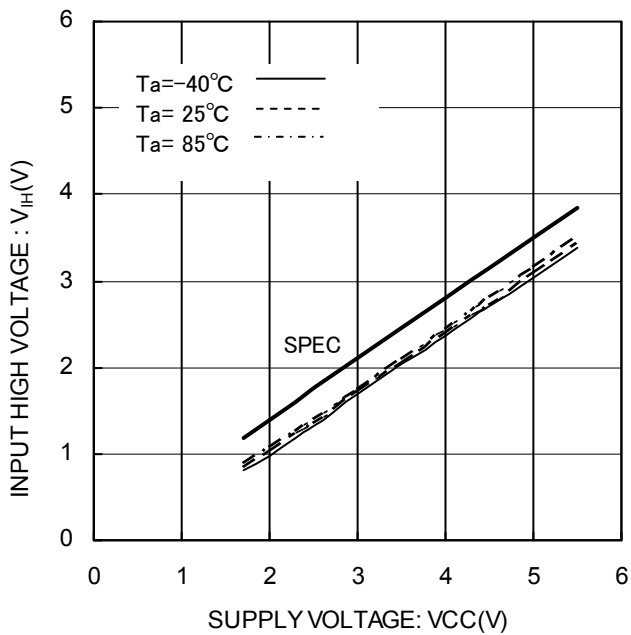
Figure 4. Input high voltage V_{IH}(\text{CS}, \text{SK}, \text{DI})
