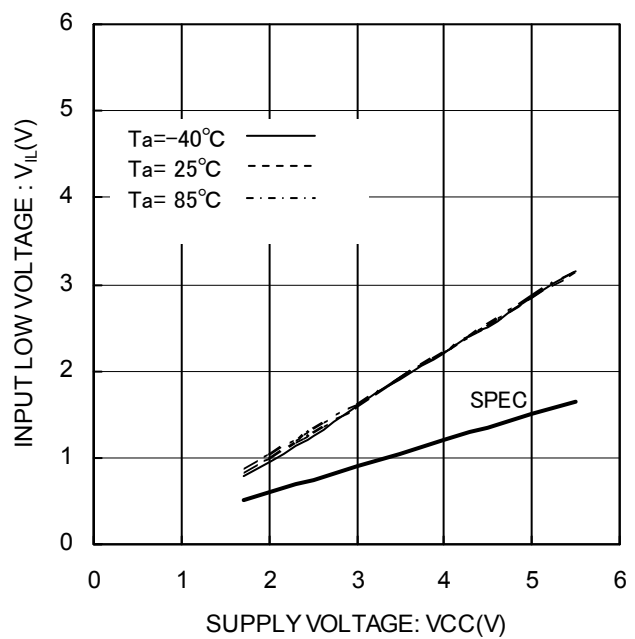
Figure 5. Input low voltage V_{IL}(\text{CS}, \text{SK}, \text{DI})
