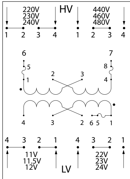
PH**QR Schematic for 50, 75 and 100VA Units
