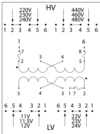
PH**QR Schematic for 150VA to 500VA Units
