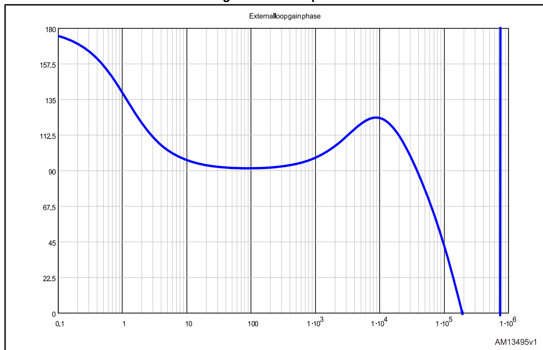
Figure 11: Phase plot
