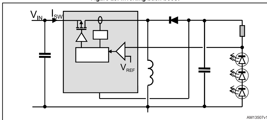
Figure 23: Inverting buck-boost
