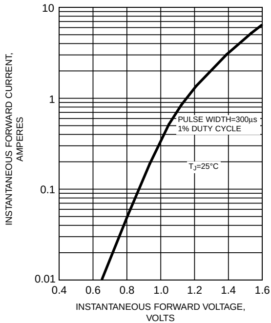
FIG. 3 - TYPICAL INSTANTANEOUS FORWARD CHARACTERISTICS FOR SML4763
