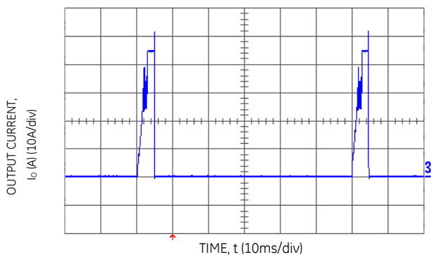
Figure 18. Output short circuit Current ( V_{in} = 12.0 Vdc, V_o = 0.75 Vdc).
