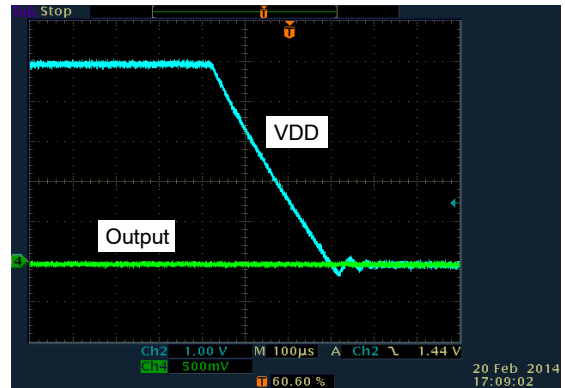
Figure 29. Output Behavior vs. Supply Voltage NCV81071B (Non-Inverting) 10 nF between Output and GND, INA = GND, ENA = VDD
