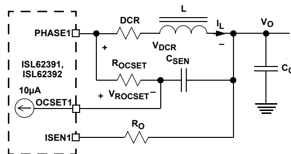
FIGURE 26. OVERCURRENT-SET CIRCUIT
