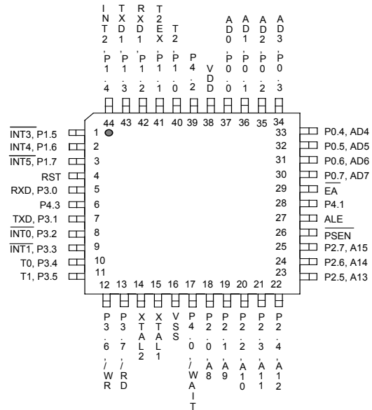
44-Pin QFP
