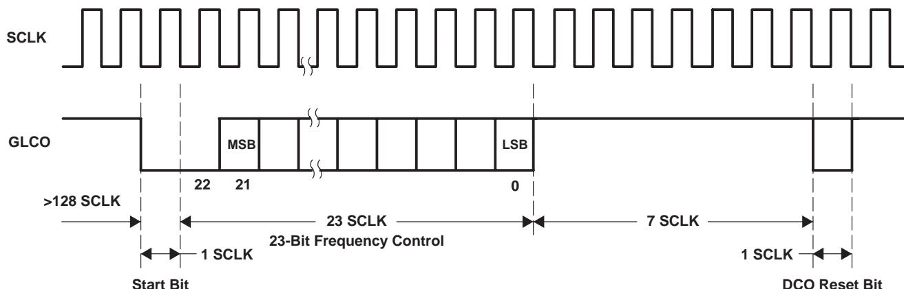
Figure 3–13. GLCO Timing
