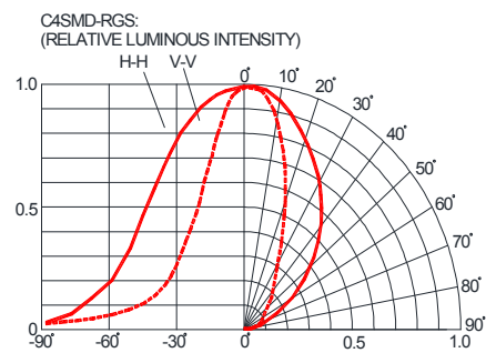
FIG.6b RED FAR FIELD PATTERN
