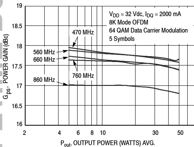
Figure 10. Single-Channel DVBT OFDM Broadband Performance Power Gain versus Output Power
