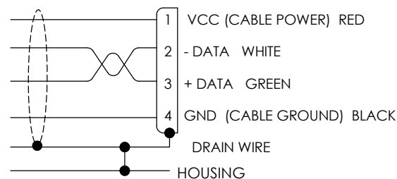
WIRING DIAGRAM "J1"
