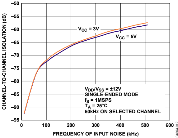
Figure 14. Channel-to-Channel Isolation
