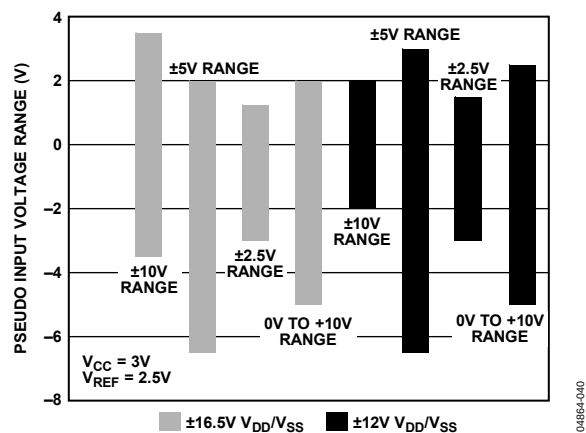
Figure 41. Pseudo Input Range with V_{CC} = 3V
