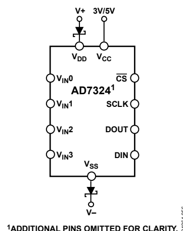
Figure 54. Schottky Diode Connection
