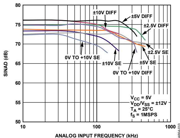
Figure 12. SINAD vs. Analog Input Frequency for Single-Ended (SE) and True Differential Mode (Diff) at 5 V CC
