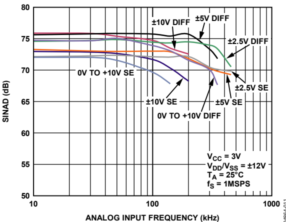
Figure 13. SINAD vs. Analog Input Frequency for Single-Ended (SE) and True Differential Mode (Diff) at 3 V CC
