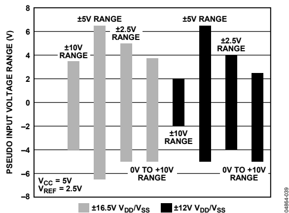
Figure 40. Pseudo Input Range with V_{CC} = 5V
