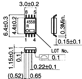
BA4558RFV(SSOP-B8) (Unit:[mm])
