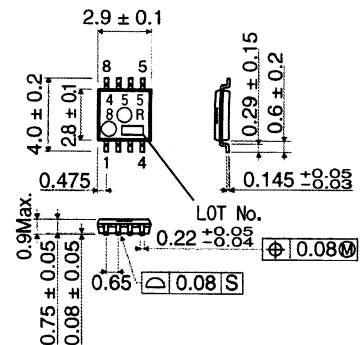
BA4558RFVM(MSOP8) (Unit:[mm])
