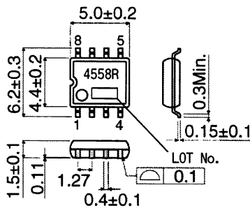
BA4558RF(SOP8) (Unit:[mm])
