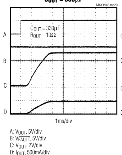
STARTUP WAVEFORMS C_{OUT} = 330\mu F
