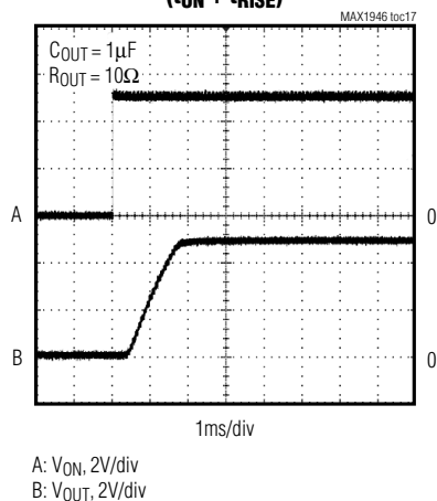
SWITCH TURN-ON TIME ( t_{ON} + t_{RISE} )
