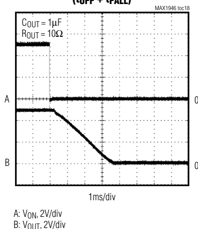
SWITCH TURN-OFF TIME ( t_{OFF} + t_{FALL} )
