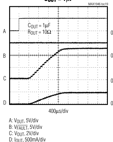
STARTUP WAVEFORMS C_{OUT} = 1\mu F
