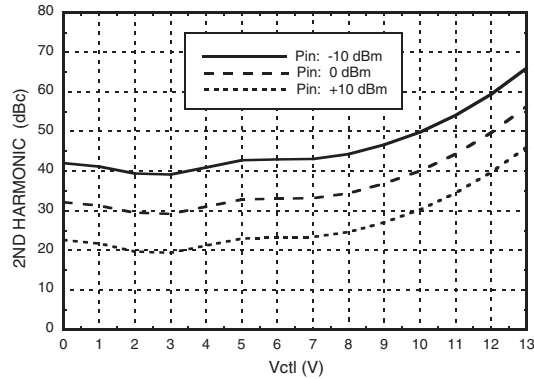
Second Harmonics vs. Vctl, F = 6 GHz
