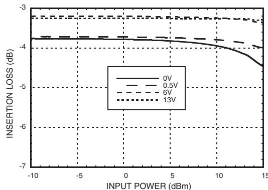
Insertion Loss vs. Pin @ 6 GHz
