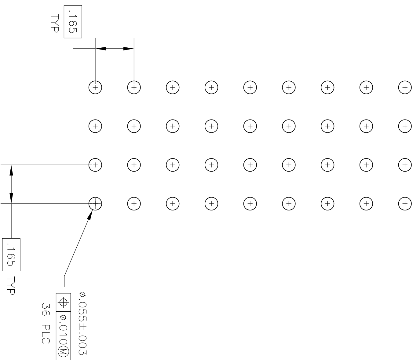
RECOMMENDED P.C. BOARD LAYOUT
