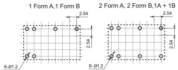
2 coils latching
