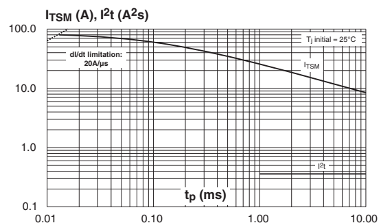
Figure 8. Non-repetitive surge peak on-state current and corresponding value of I^2t sinusoidal pulse width
