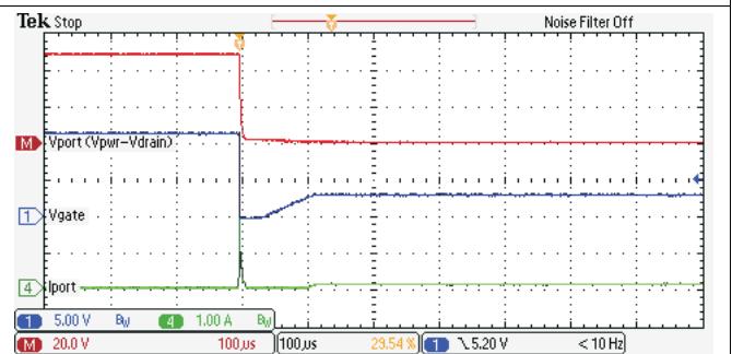
Figure 28. Rapid Response to a 1-Ω Short: PoE+ Mode
