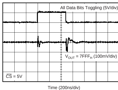
DIGITAL FEEDTHROUGH
